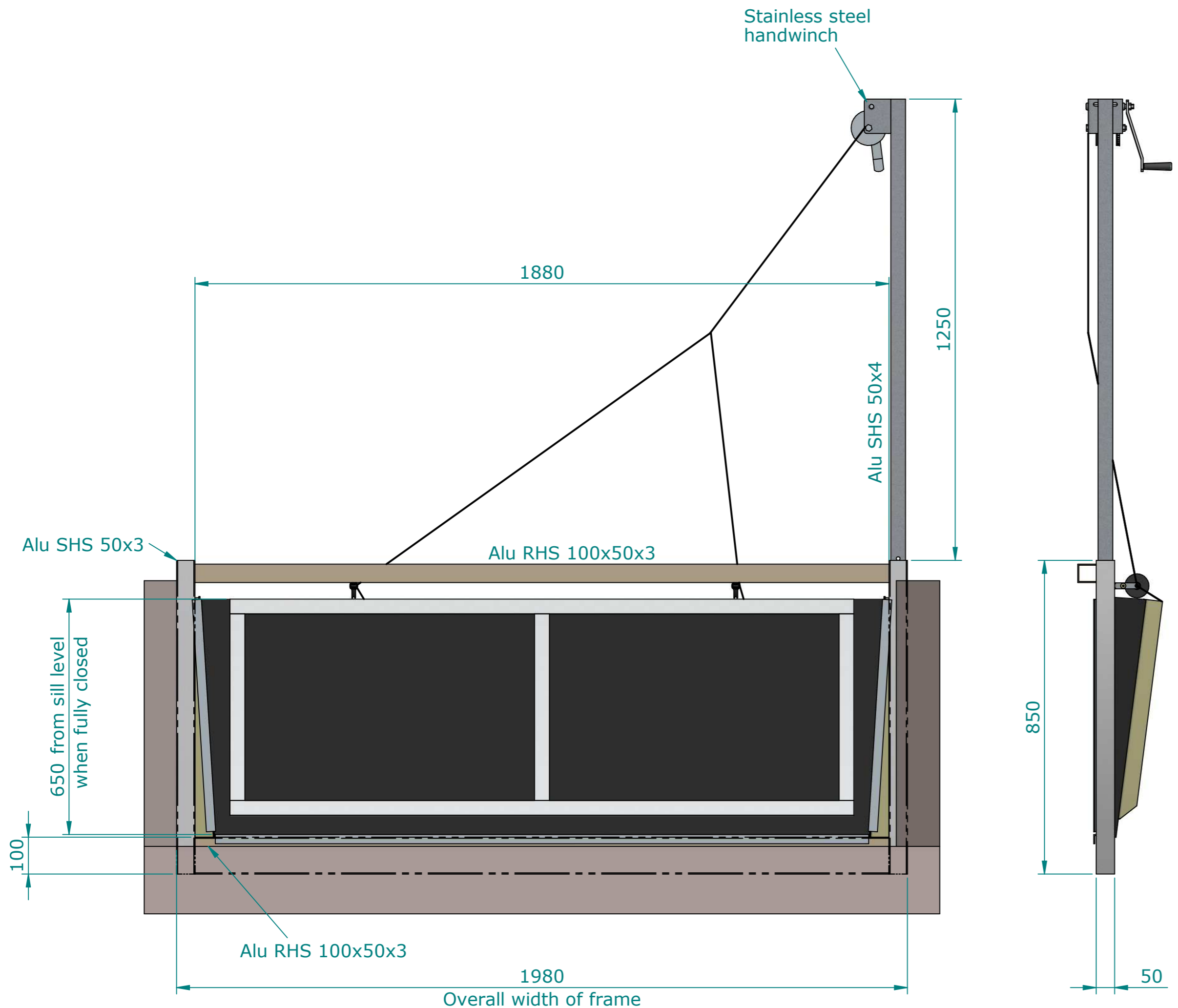
Prawn Door Aluminium Front view, Scale 1:10
